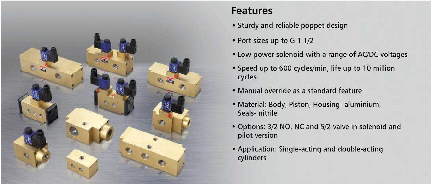
5/2 Single Solenoid
